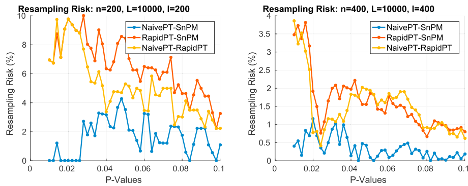
Fig. 11. Resampling risk of NaivePT-SnPM, RapidPT-SnPM, and NaivePT-RapidPT. The hyperparameters used were: \eta = 0.35\% , L = 10000 , and l = n .
