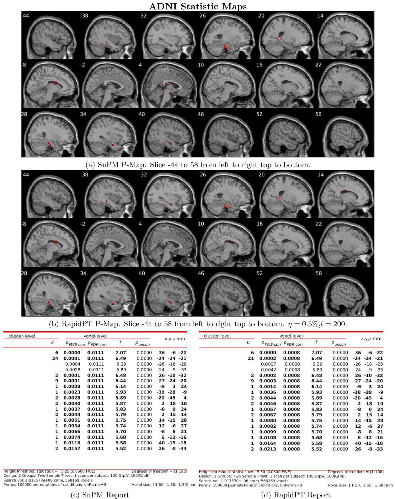
Fig. 10. Thresholded FWER corrected statistical maps at ( \alpha = 0.05 ) with the n = 200 dataset. The hyperparameters used were: \eta = 0.5\% , l = n , and L = 100000 . The images show the test statistics for which the null was rejected in SnPM (top) and RapidPT (bottom). The tables show a numerical summary of the images. The columns refer to: k - cluster size, P_{FWE-corr} -
