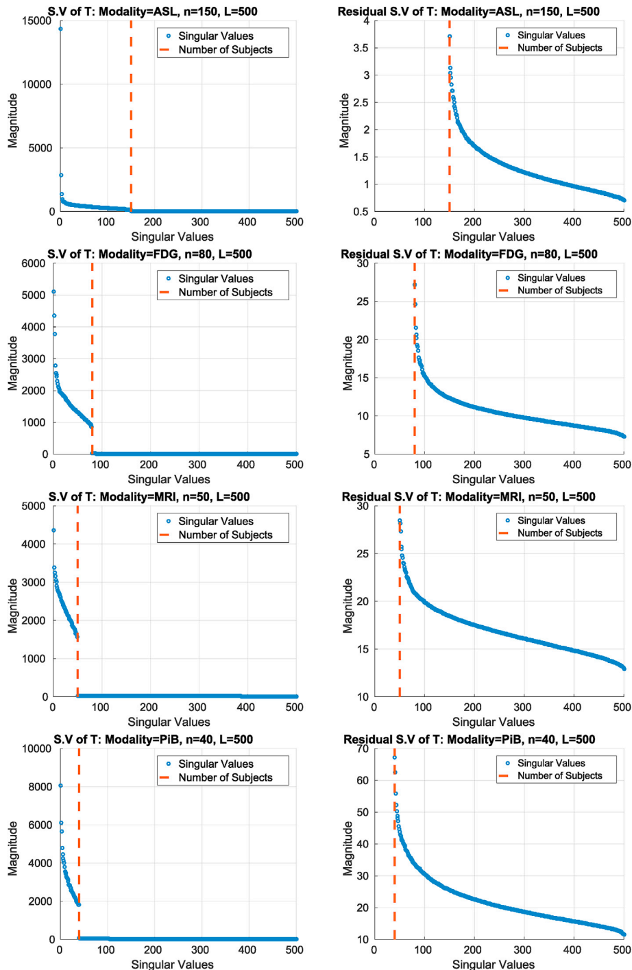
Fig. 2. Singular value spectra for permutation testing matrices with dimensions generated from the imaging modalities: ASL, FDG PET, MRI, and PiB PET. Left: Full spectrum of T with L rows and v columns. Right: Residual singular values of T .
