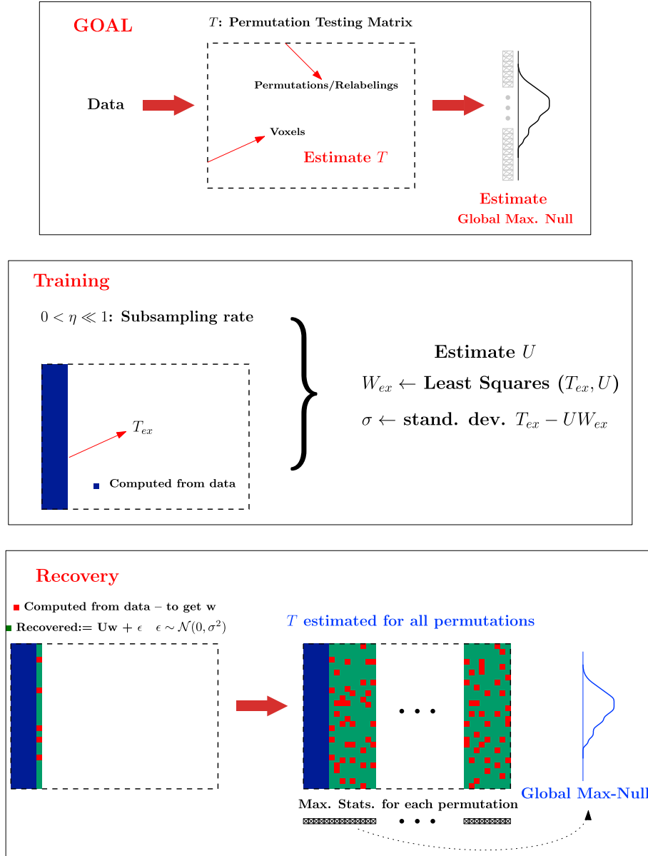
Fig. 3. Flow diagram of the training and recovery steps in RapidPT. The number of training samples ( l ) and the rank of U(r) is the number of columns computed in the training phase (the blue area). The sub-sampling rate, \eta , is the fraction of red over green entries computed per column. The global max null is h^t in the algorithm.
