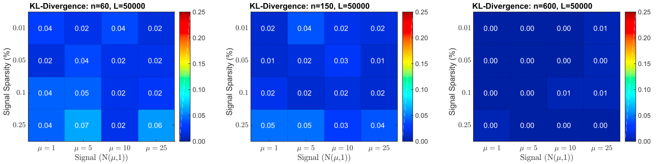
Fig. 6. KL-Divergence between the true max null and the one recovered by RapidPT on 48 datasets. The sub-sampling rate, \eta , used for each run was 2\eta_{min} . The number of training samples, l , used for each run was n (i.e., the same as the number of images in the dataset).
